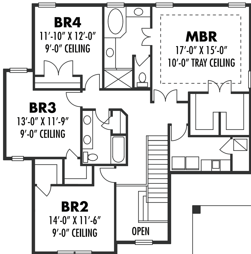
UPPER FLOOR
