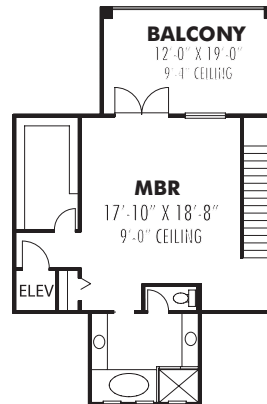
TOP FLOOR PLAN
