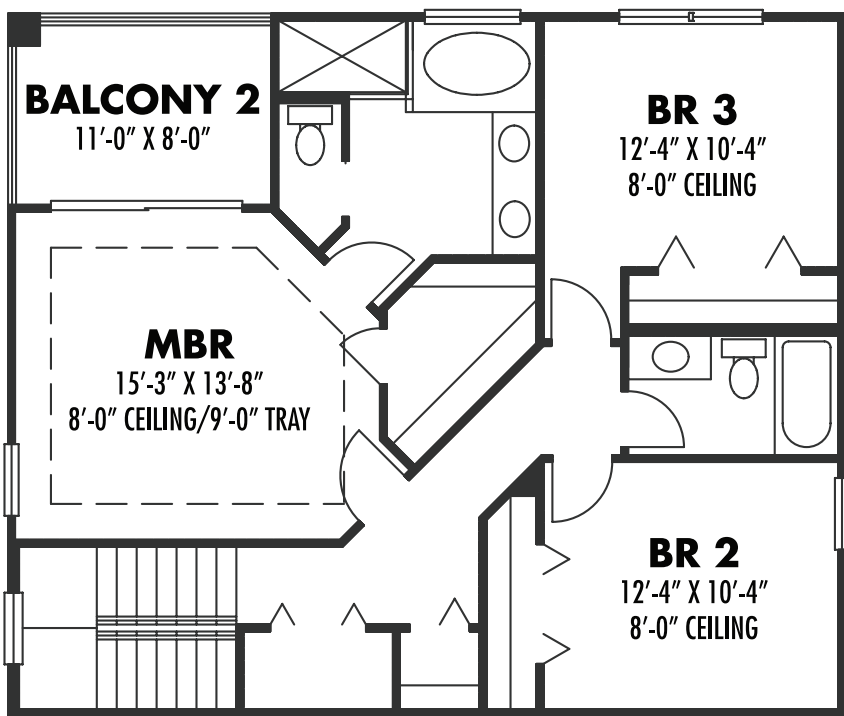
TOP FLOOR PLAN
