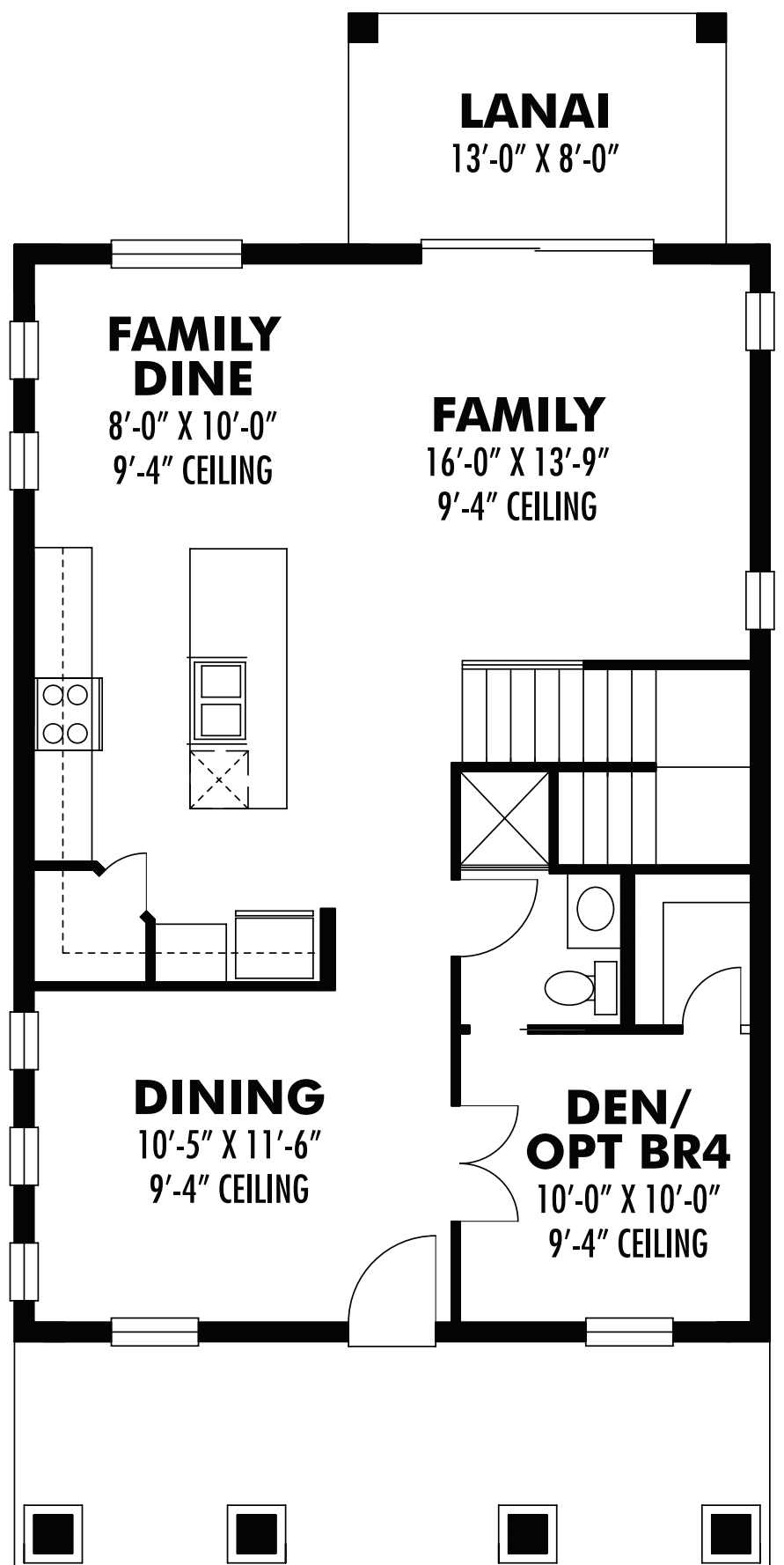
MAIN FLOOR PLAN
