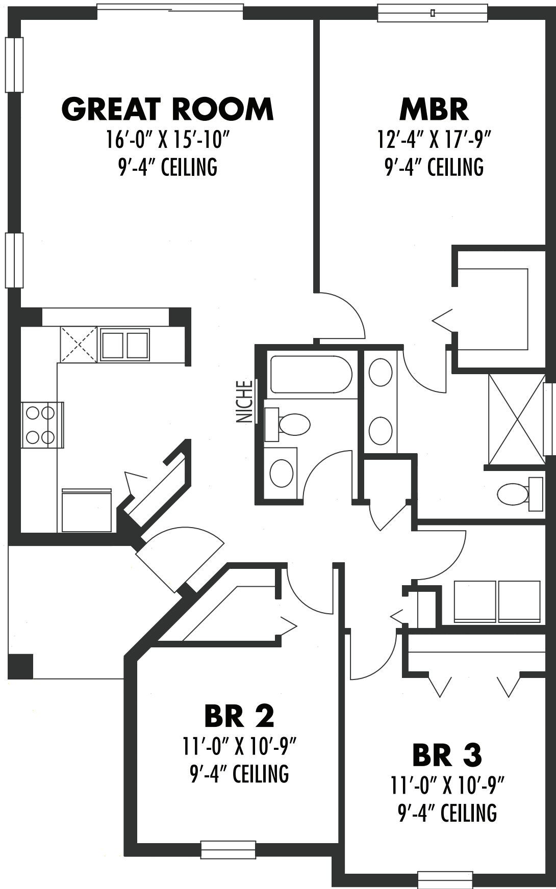
PLAN 1293 1293 SQUARE FEET 30'-0" x 48'-0" 9'-4" CEILINGS SLAB FOUNDATION
