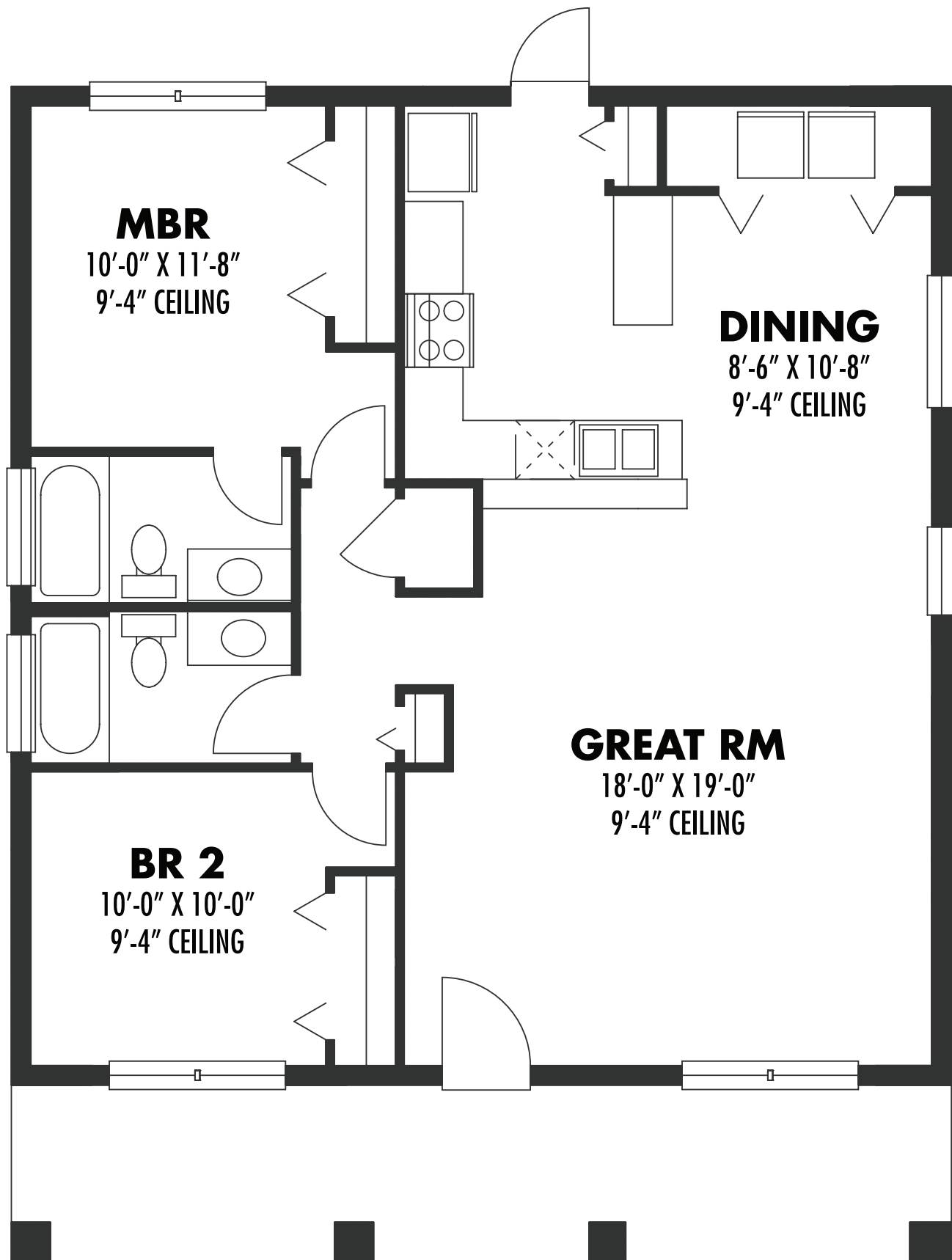
PLAN 1088 1088 SQUARE FEET 32'-0" X 40'-0" 9'-4" CEILINGS SLAB FOUNDATION
